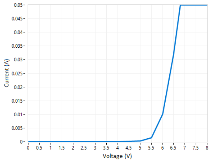
Figure 4. Forward current vs forward voltage T_s=25\text{ }^\circ\text{C}
