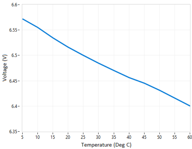
Figure 7. Forward voltage vs temperature I_F = 20 \text{ mA}
