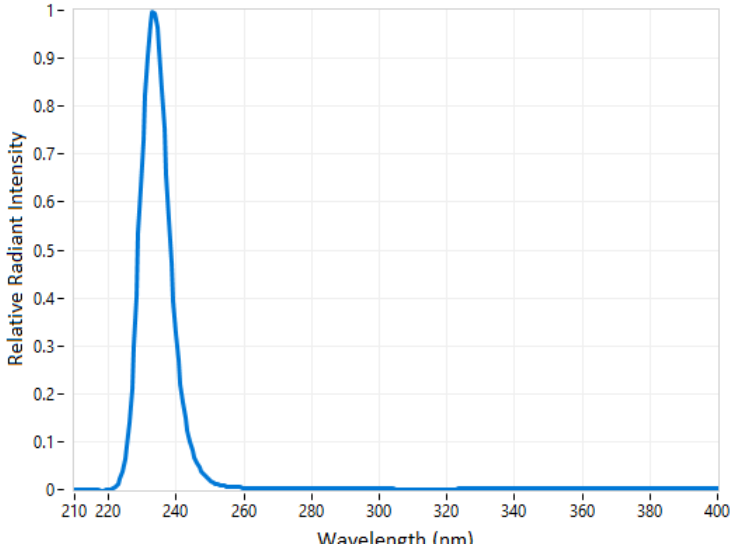
Figure 1. Relative emission intensity vs wavelength T_s=25\text{ }^\circ\text{C} , I_f = 20\text{ mA}
