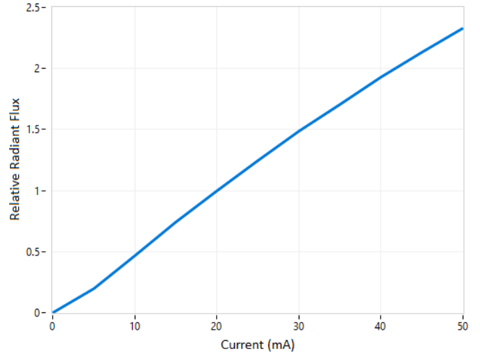
Figure 2. Relative radiant flux vs forward current T_s=25\text{ }^\circ\text{C}
