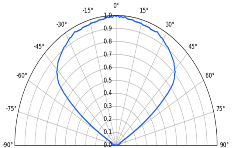
Figure 8. Radiation pattern T_A = 25 \text{ °C}, I_F = 20 \text{ mA}
