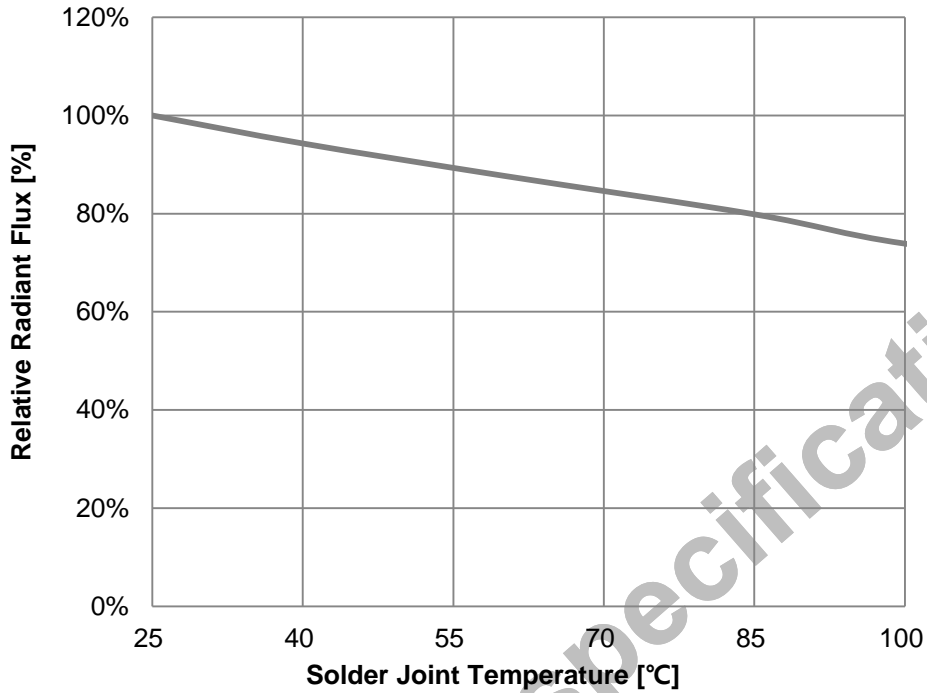
Fig 5. Ambient Temperature vs. Relative Radiant Flux, I_F=100mA
