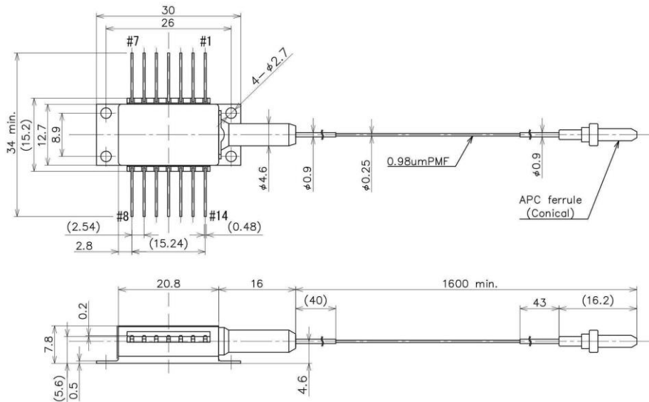
(b) 250um fiber diameter and ferrule type (QLD1a61-xyyPzWtt11)
