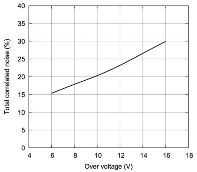
Figure 11: Total Correlated Noise vs. Overvoltage
