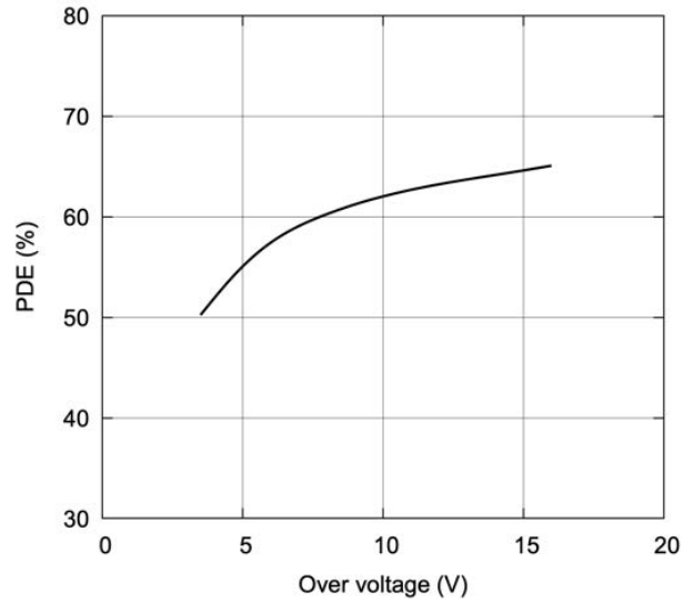
Figure 7: PDE vs. OV at 420 nm
